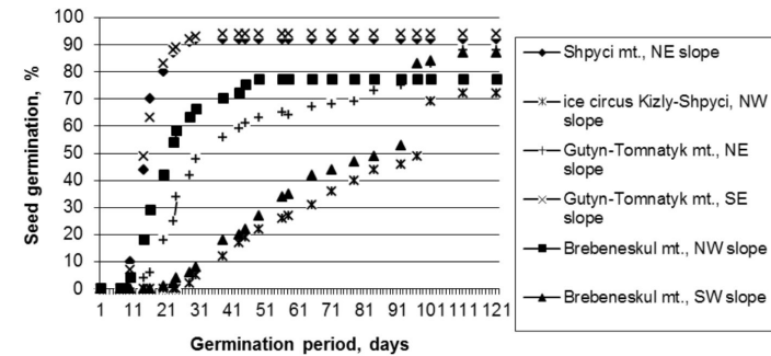
Fig. 3. Dynamics of seed germination of Loiseleuria procumbens (L.) Desv. from several habitats
